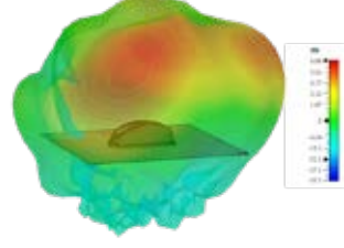
3D Plot Element 4 Side (2000 MHz)
